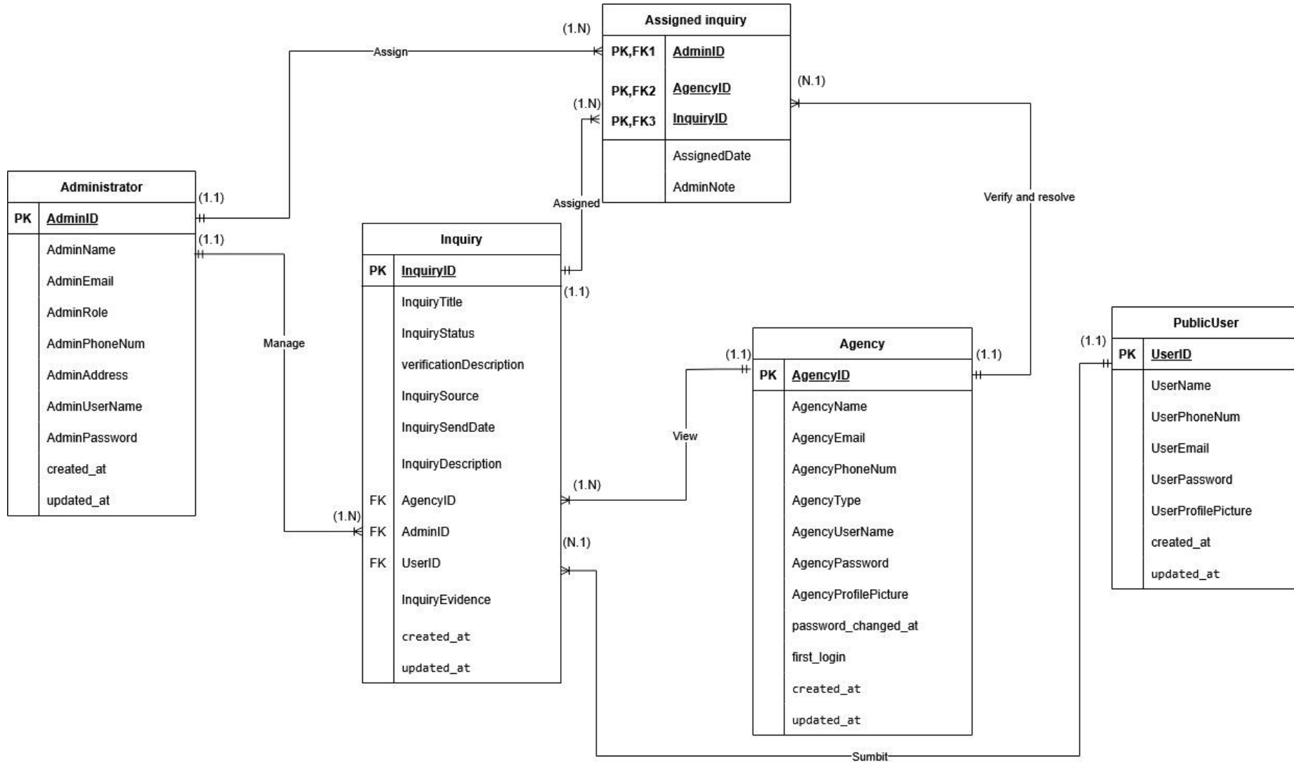
Figure 2.1 Entity Relationship Diagram (ERD) for AuthenticityHub System
