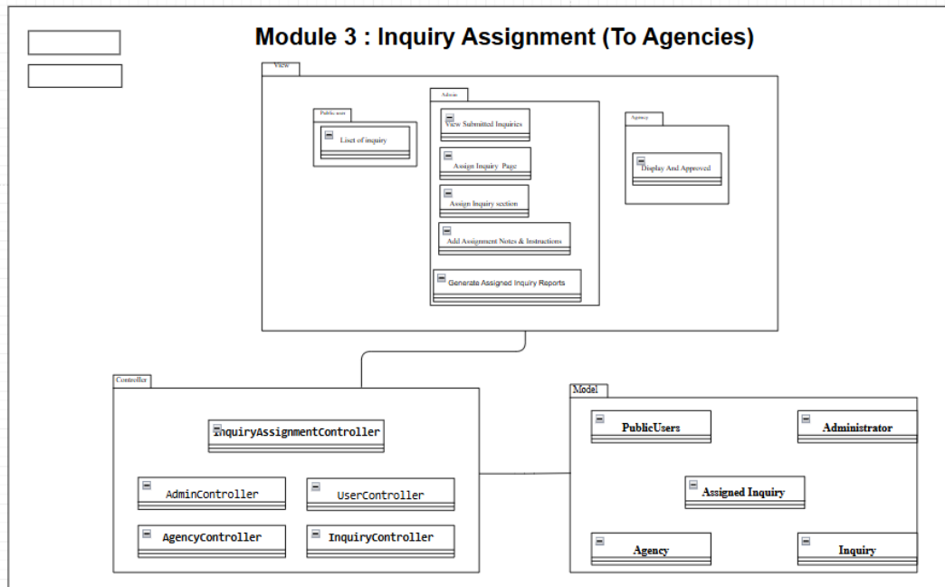
Figure 3.2.3 Component Module 3: Inquiry Assignment (to Agencies)
