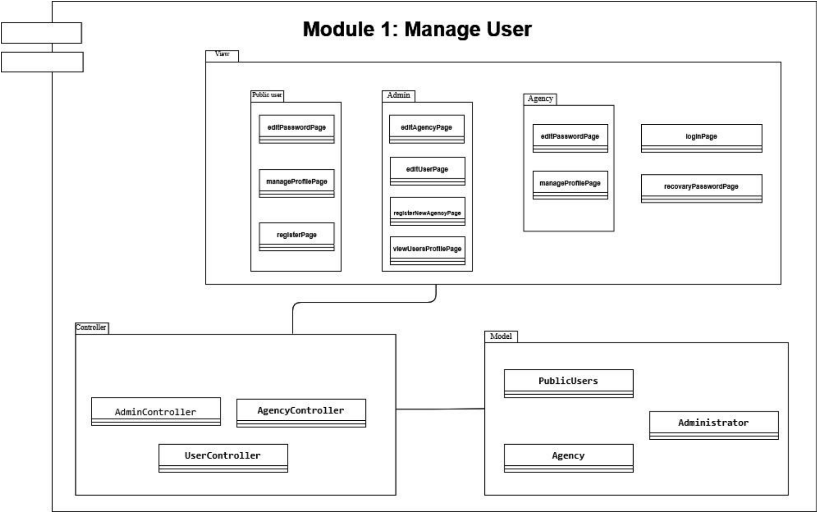
Figure 3.2.1 Component Module 1: Manage Use
