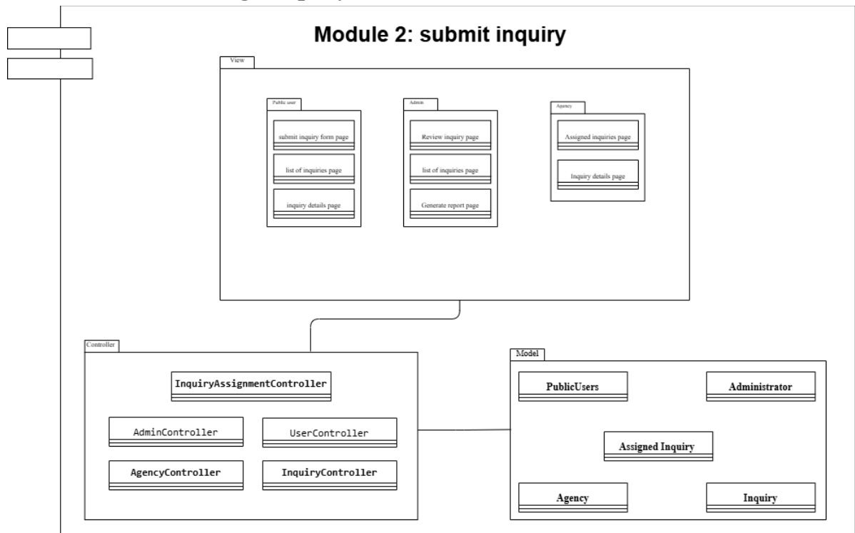
Figure 3.2.2 Component Module 2: Manage Inquiry Form Submission
