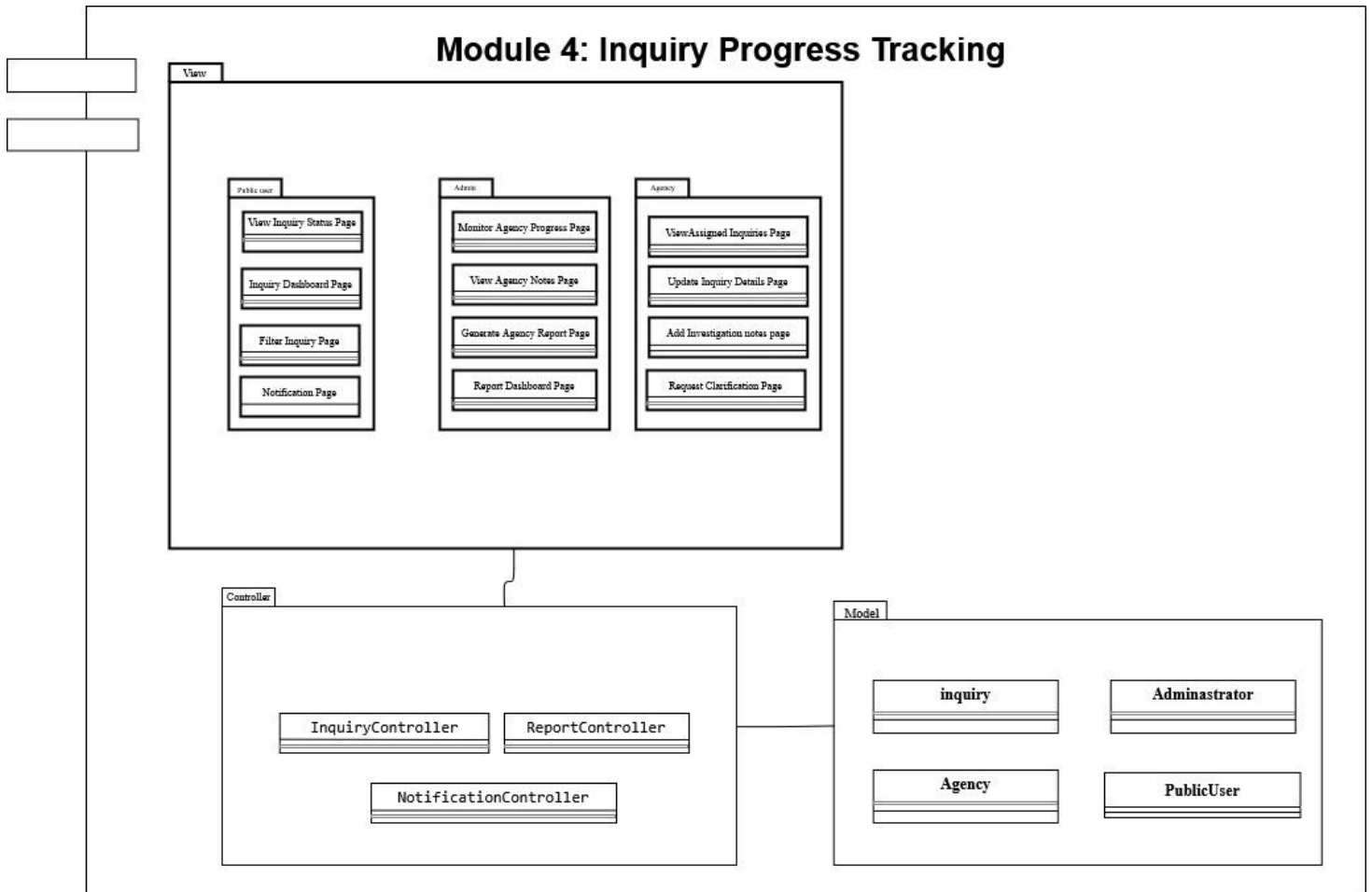
Figure 3.2.4 Component Module 4 Inquiry Progress Tracking
